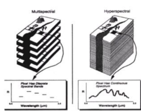
Figure 2: Example of the spectral information contained in an MSI and a HSI pixel (source https://www.sfpt.fr ).
