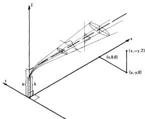
Gaussian Plume (source: Turner, 1994)
