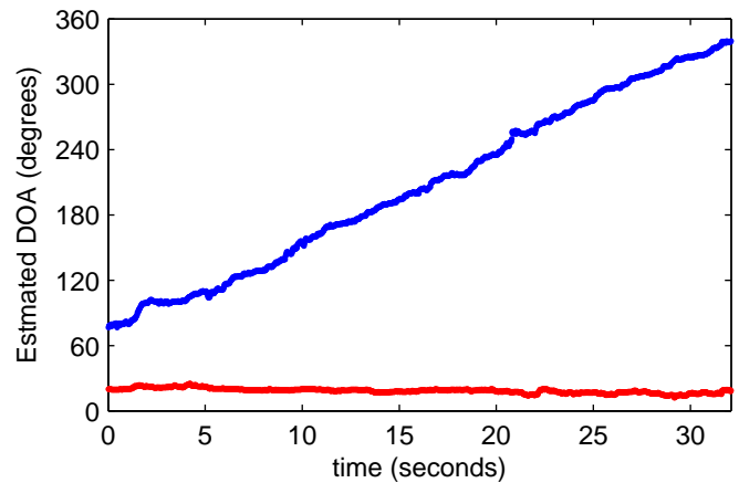
Fig. 7. DOA estimation over time for recordings of one moving and one static speaker, who both speak continuously and simultaneously, using the proposed method.
