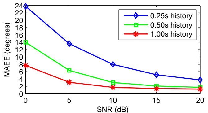
Fig. 5. DOA estimation error vs SNR for four intermittent speakers simulated reverberant environment.
