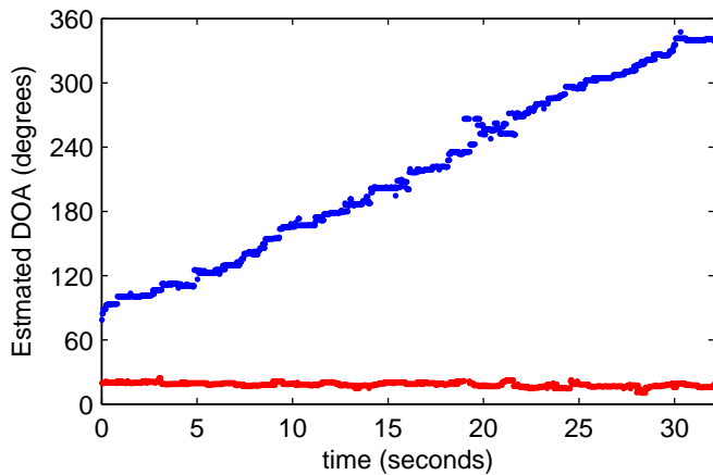
Fig. 6. DOA estimation over time for recordings of one moving and one static speaker, who both speak continuously and simultaneously, using the method of [8].
