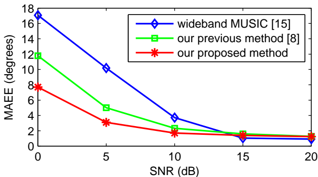
Fig. 3. DOA estimation error vs SNR for four intermittent speakers in a simulated reverberant environment.
